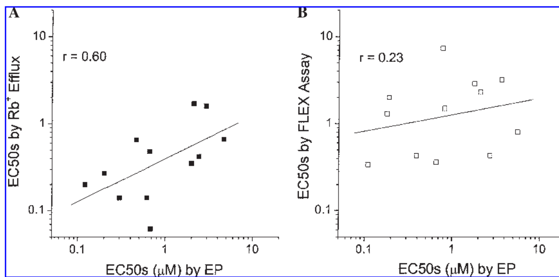
FIG. 7. EC_{50} correlation between Rb^+ efflux assay and EP. (A) Correlation of EC_{50} values of WAY compounds determined by whole-cell recordings and Rb^+ efflux assay. The EC_{50} values from both assays agreed each other with a correlation coefficient of 0.6. (B) The same set of compounds was also evaluated using membrane potential dye-based FlexStation assay. The comparison of values from EP and FlexStation assays showed no correlation ( r = 0.23 ).
