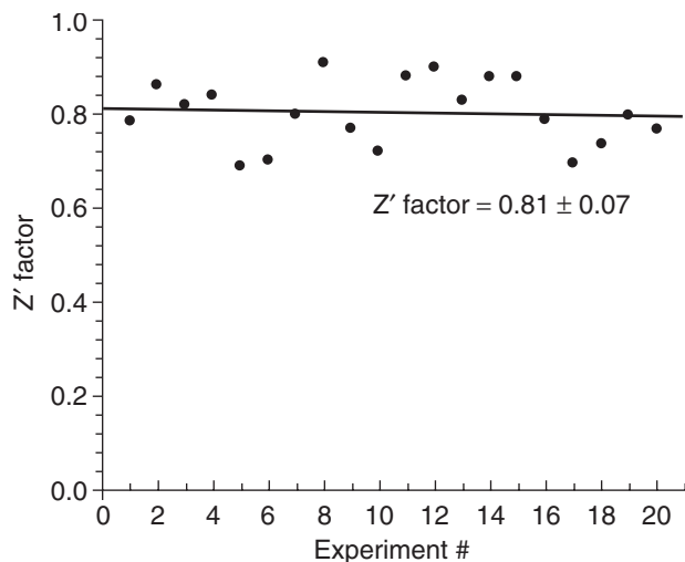
FIG. 8. Performance of atomic absorption Rb + efflux assay. Z' factor for each experiment was determined from positive (in the presence of 1 \mu M KCNQ-channel opener compound) and negative (in the absence of compound) controls. The values of Z' ranged from 0.7 to 0.91 with an average of 0.81 \pm 0.07.
