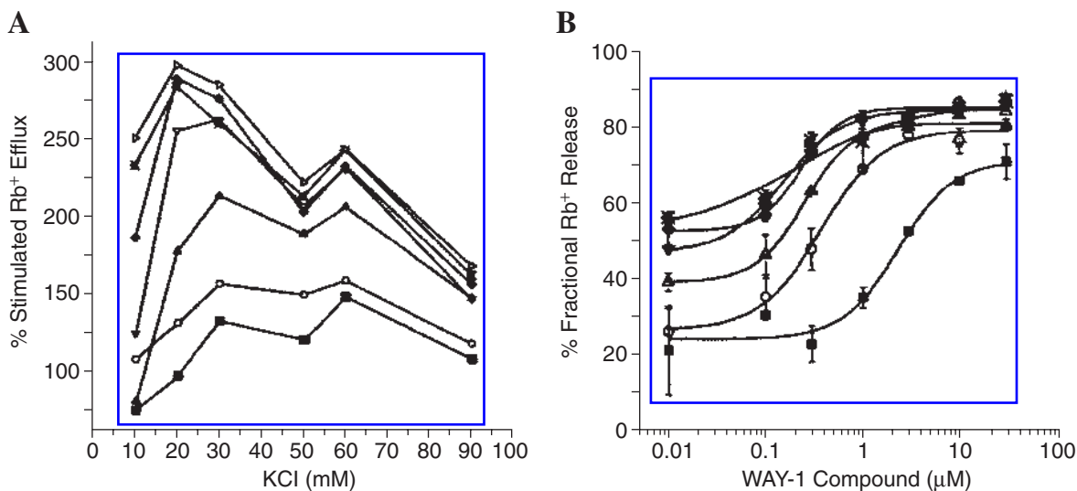
FIG. 2. Effect of extracellular K + concentration on Rb + release in the presence of a KCNQ channel opener (WAY-1 compound). (A) Rb + efflux stimulated by extracellular K + from 10 to 90 mM in the presence of WAY-1 compound from 0.01 to 30 µM (■, 0.01 µM; ○, 0.1 µM; △, 0.3 µM; ▽, 1.0 µM; ◇, 3.0 µM; ⋈, 10 µM; △, 30 µM). Depolarization with 20 mM KCl produces the maximal Rb + efflux in the presence of the WAY-1 with the biggest assay window (200%), compared with 175% for 10 mM or lower for 30–90 mM KCl under isosmotic conditions. (B) EC 50 values (µM) of WAY-1 compound determined from A and plotted for different concentrations of KCl are 2.29, 0.37, 0.25, 0.16, 0.24, and 0.22 for 10 mM (■), 20 mM (○), 30 mM (△), 50 mM (▽), 60 mM (◇), and 90 mM (⋈), KCl, respectively.
