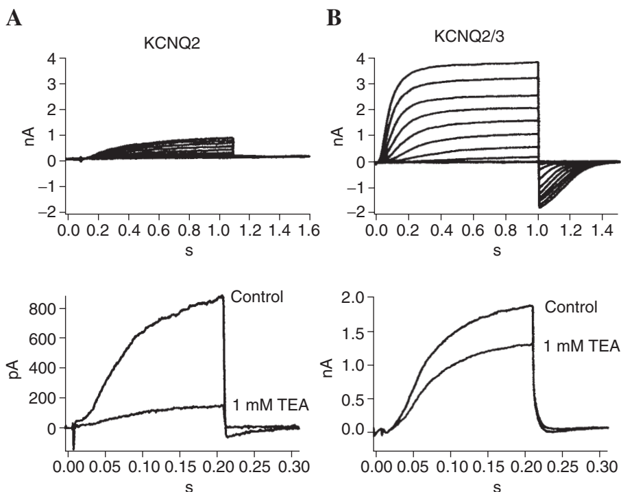
FIG. 1. Functional and pharmacological confirmation of stable KCNQ2/3 CHO cells. (A) KCNQ2 current traces in a cell held at -80 mV (top panel) were elicited with 1.0-s depolarizing pulses in 10-mV increments from -80 to +20 mV. The bottom panel shows the block of KCNQ2 current by TEA (1.0 mM). (B) KCNQ2/3 current traces were elicited with the same protocol used in A. The bottom panel displays the current block by TEA (1.0 mM).
