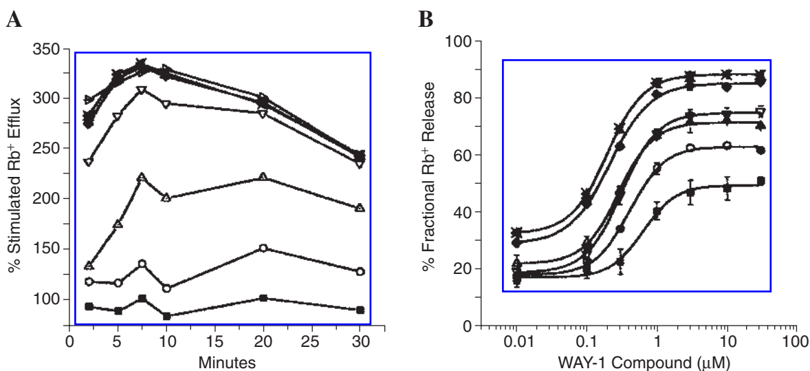
FIG. 3. Time course of Rb + release following depolarization (by 20 mM KCl) in the presence of WAY-1 compound. (A) Time course of Rb + efflux at different concentrations of WAY-1 compound from 0.01 to 30 µM (■, 0.01 µM; ○, 0.1 µM; △, 0.3 µM; ▽, 1.0 µM; ◇, 3.0 µM; ⋈, 10 µM and ▷, 30 µM). (B) Concentration-response curves for WAY-1 compound at different time points from 2 to 30 min (■, 2 min; ○, 5 min; △, 7.5 min; ▽, 10 min; ◇, 20 min, and ⋈, 30 min) after KCl depolarization. EC 50 values for 7.5 and 10 min were 284 nM and 315 nM, respectively, and are consistent with that obtained by EP.
