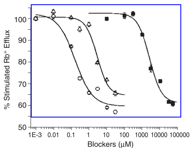
FIG. 5. Rb + efflux through KCNQ2/3 channels is blocked by K + -channel blockers. TEA (■), linopirdine (△), and XE991 (○) were added to KCNQ2/3 CHO cells during the last 30 min of Rb + loading (3 h). IC 50 values for TEA, linopirdine, and XE991 were 2.52 mM, 2.85 µM, and 0.16 µM, respectively.
