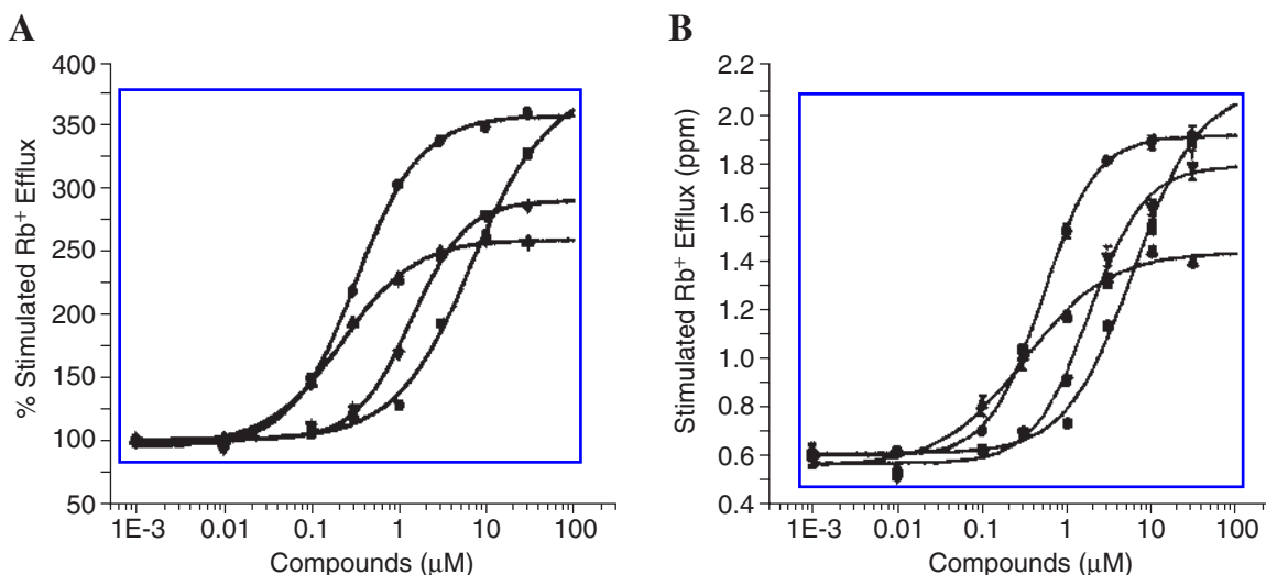
FIG. 4. Dose-dependent effects of KCNQ-channel openers on stimulated Rb + efflux. Compounds were measured in quadruplicates. (A) EC 50 values (µM) obtained from measurements of supernatant/lysate were 6.9 for WAY-2 (■), 0.33 for WAY-3 (○), 0.22 for WAY-4 (▲), and 1.4 for WAY-5 (▽). (B) Data from A were plotted for supernatant measurement only, and absolute release of Rb + was detected in the range of 0.6–2.0 ppm in response to different concentrations of the same set of compounds. EC 50 values (µM) of WAY-2 (■), WAY-3 (○), WAY-4 (▲), and WAY-5 (▽) were 6.0, 0.52, 0.32, and 1.82, respectively.
